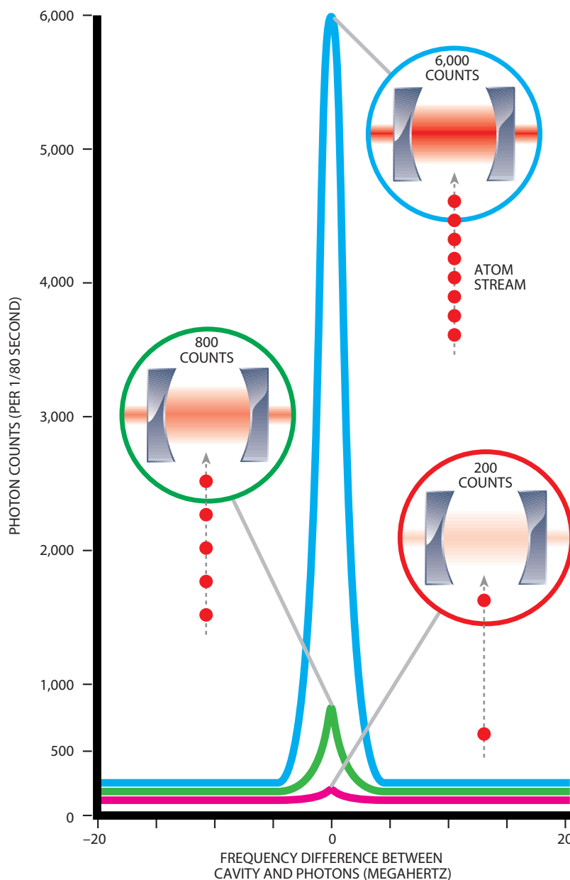
BEAM INTENSITY of the single-atom laser rises sharply when a dense stream of barium atoms enters the resonator. When the beam of atoms is sparse, laser output is much lower. Note that the photon count falls to a background level when the resonant frequency of the cavity does not match the frequency of the emitted photons.
